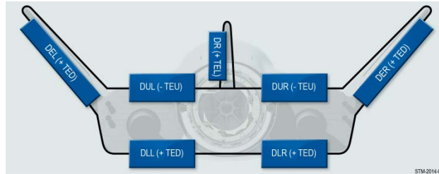
Figure 7. Dream Chaser Control Surfaces: The Dream Chaser features seven control surfaces shown here from the rear of the airframe.
